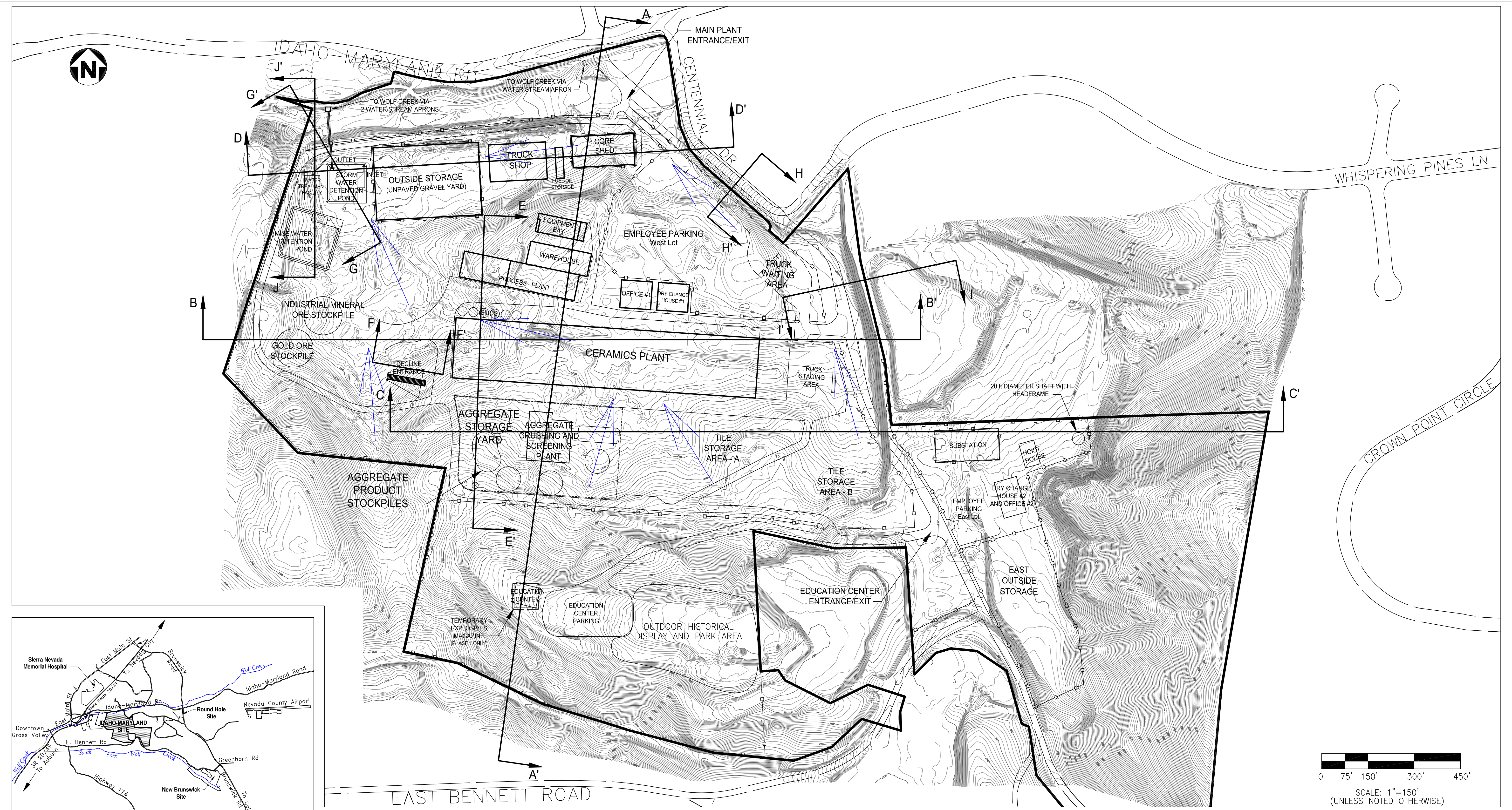
KEY PLAN
